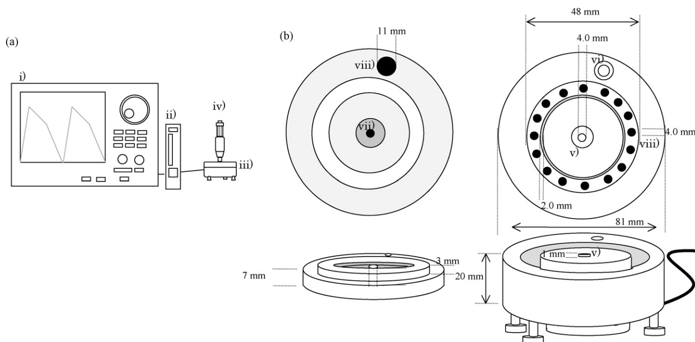
Fig. 2. Setup for TX-9A system to detect injection force of Shimajet®. (a) TX-9 system: (i) digital oscilloscope, (ii) sensor amplifier, (iii) TX-9UA, (iv) Shimajet®. (b) Diagram of TX-9: (v) load cell, (vi) level gauge, (vii) injection port, (viii) pore.
