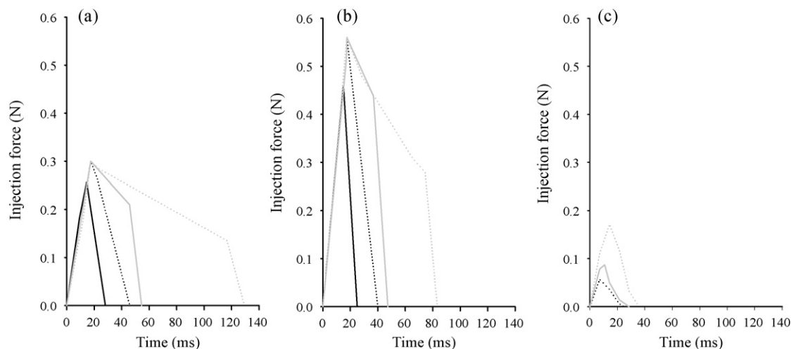
Fig. 3. Effect of nozzle type and injection volume on the time course of injection force after injection by ShimaJet®. (a) NFI-w with normal nozzle, (b) NFI-s with normal nozzle, (c) NFI-s with modified nozzle; Lines: —: 50 µL, ....: 100 µL, ———: 125 µL, ●●●●●: 250 µL for injection volume.
