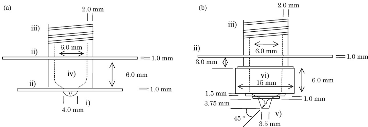
Fig. 1. Diagram of normal and modified nozzles of ShimaJet®. (a) Commercially available disposal nozzle: (i) injection port, (ii) nozzle-fixing bar, (iii) screw thread, (iv) solution-filling space. (b) Modified nozzle: (v) injection port, (vi) solution-filling space made of brass.
